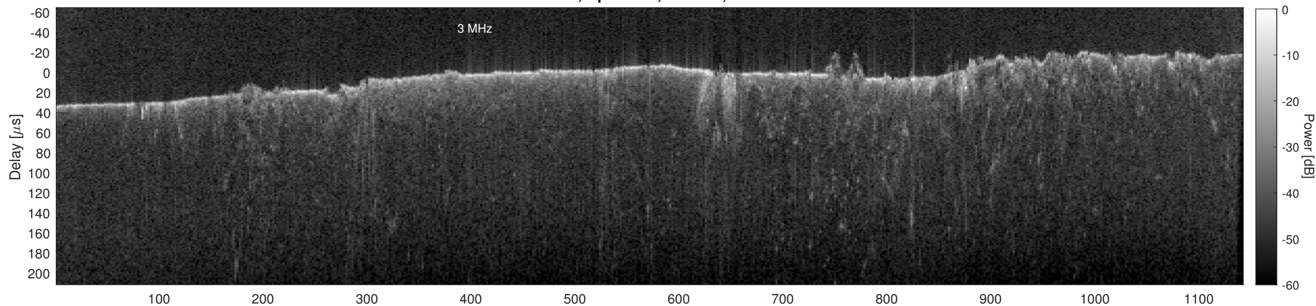
Orbit 13322, Cluttergram
