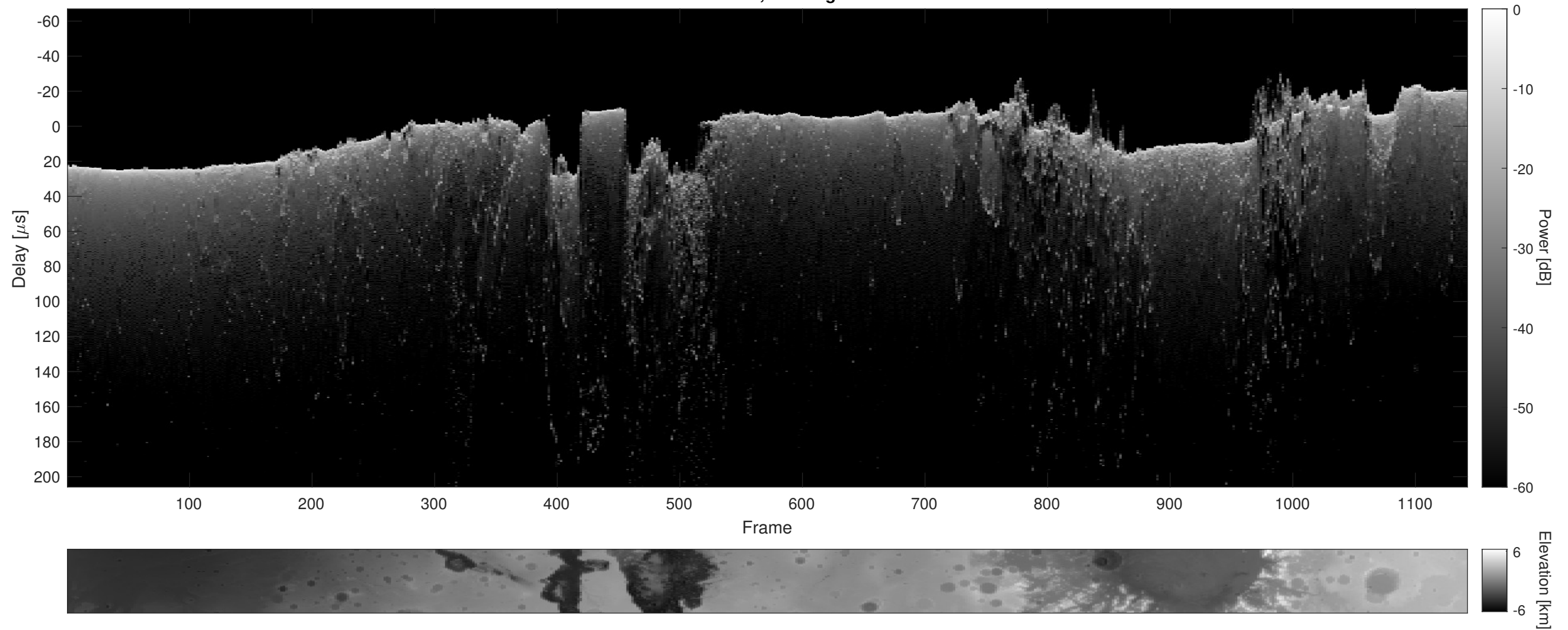
Orbit 13327, Cluttergram
