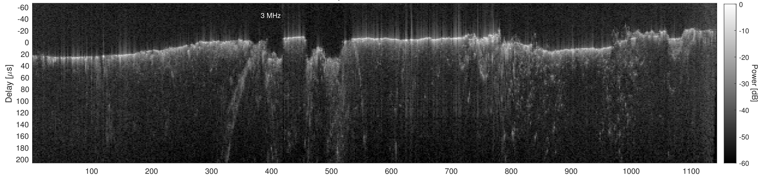
Orbit 13327, Cluttergram
