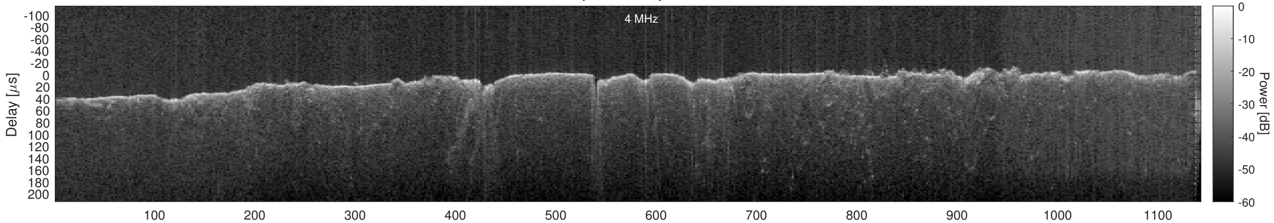
Orbit 13329, Window, Channel 1, Chapman
