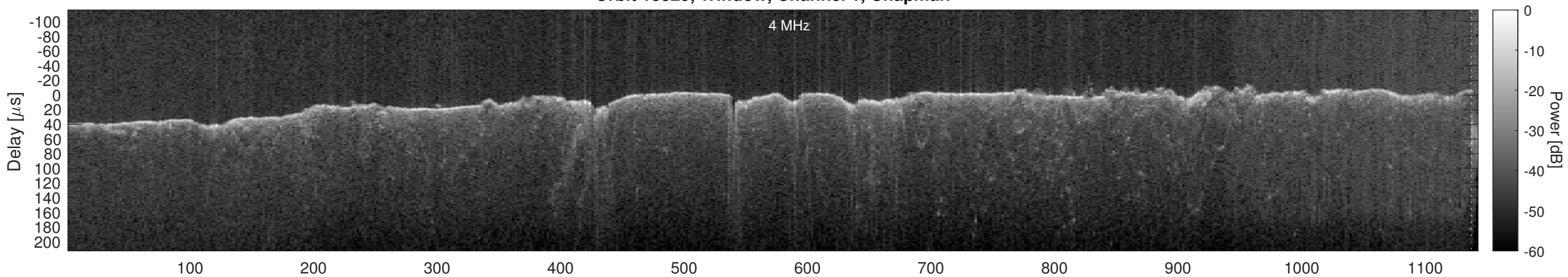
Orbit 13329, Window, Channel 1, Optimized
