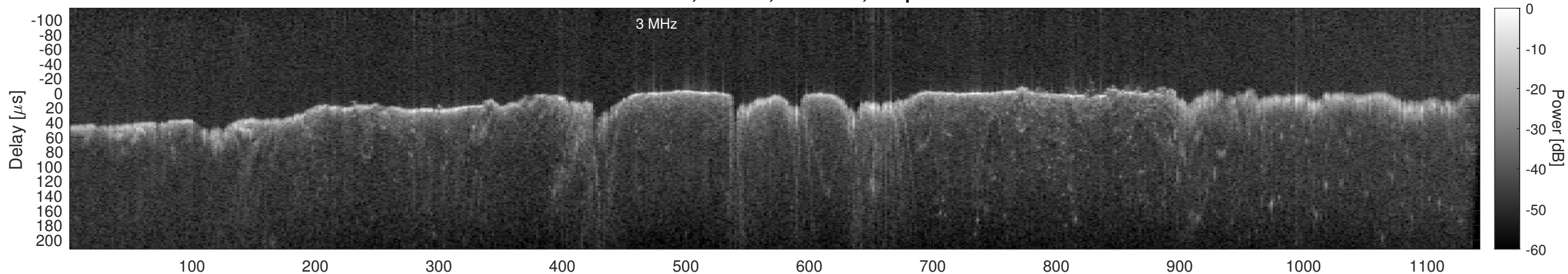
Orbit 13329, Window, Channel 2, Optimized
