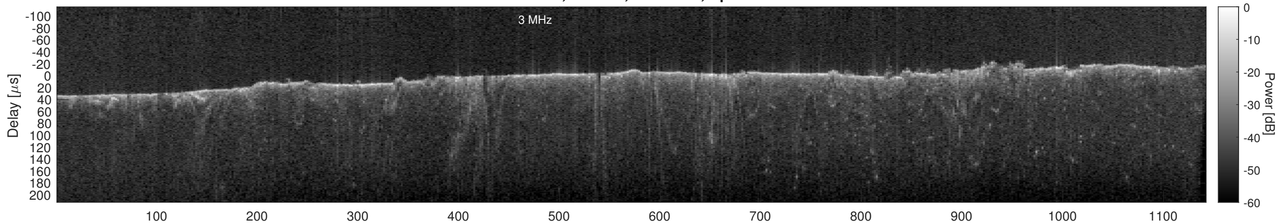
Orbit 13329, Cluttergram
