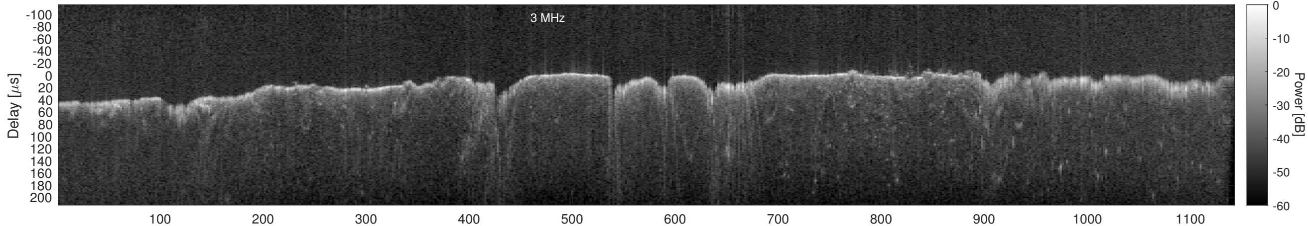
Orbit 13329, Window, Channel 2, Chapman
