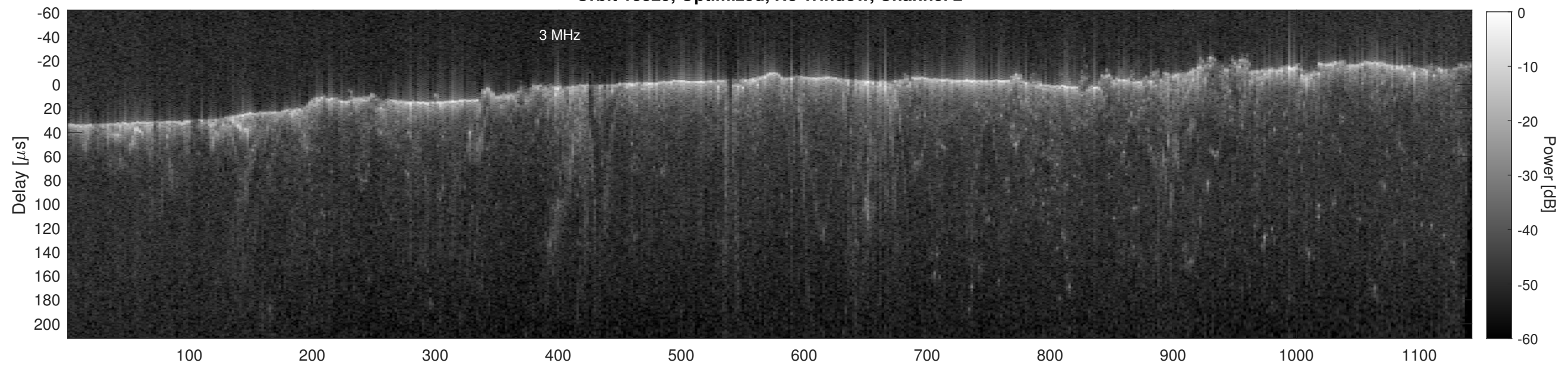
Orbit 13329, Cluttergram
