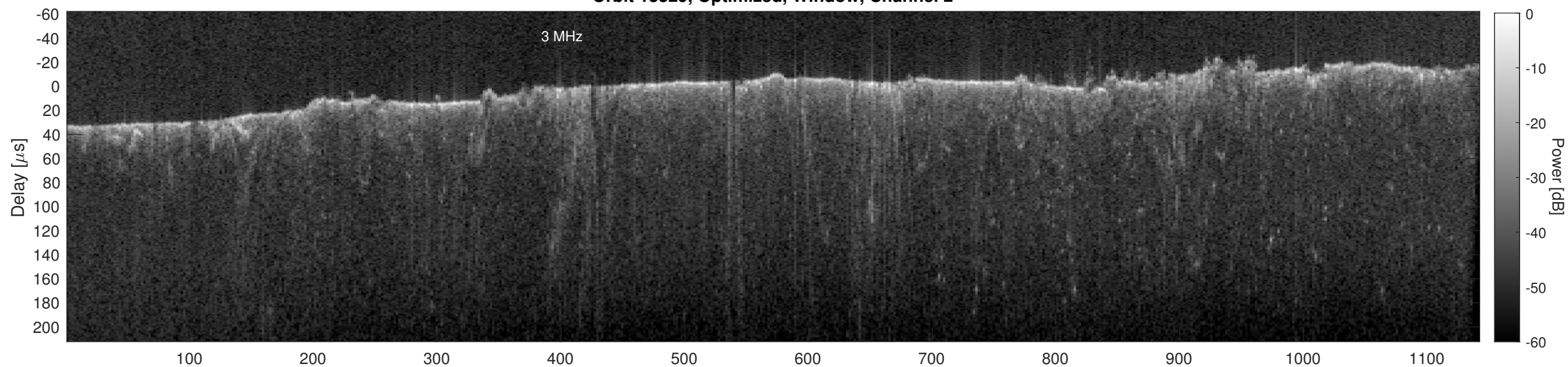
Orbit 13329, Cluttergram
