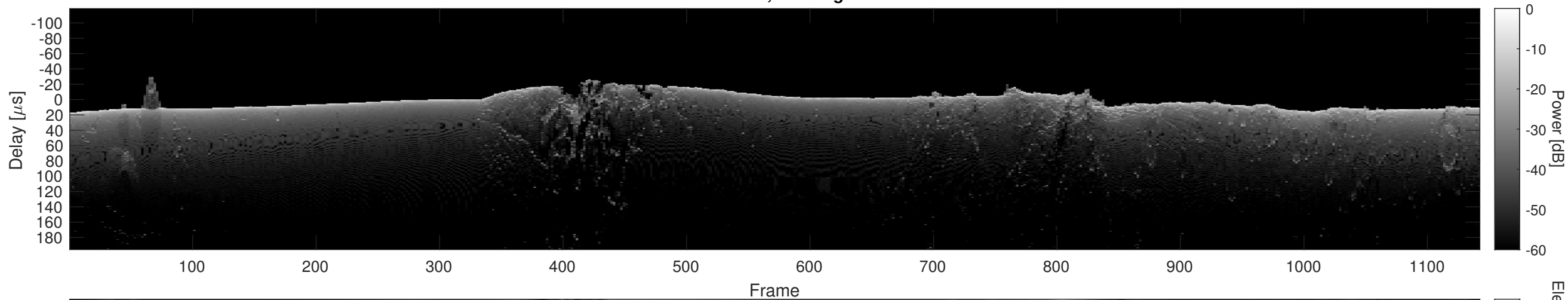
Orbit 13331, Cluttergram
