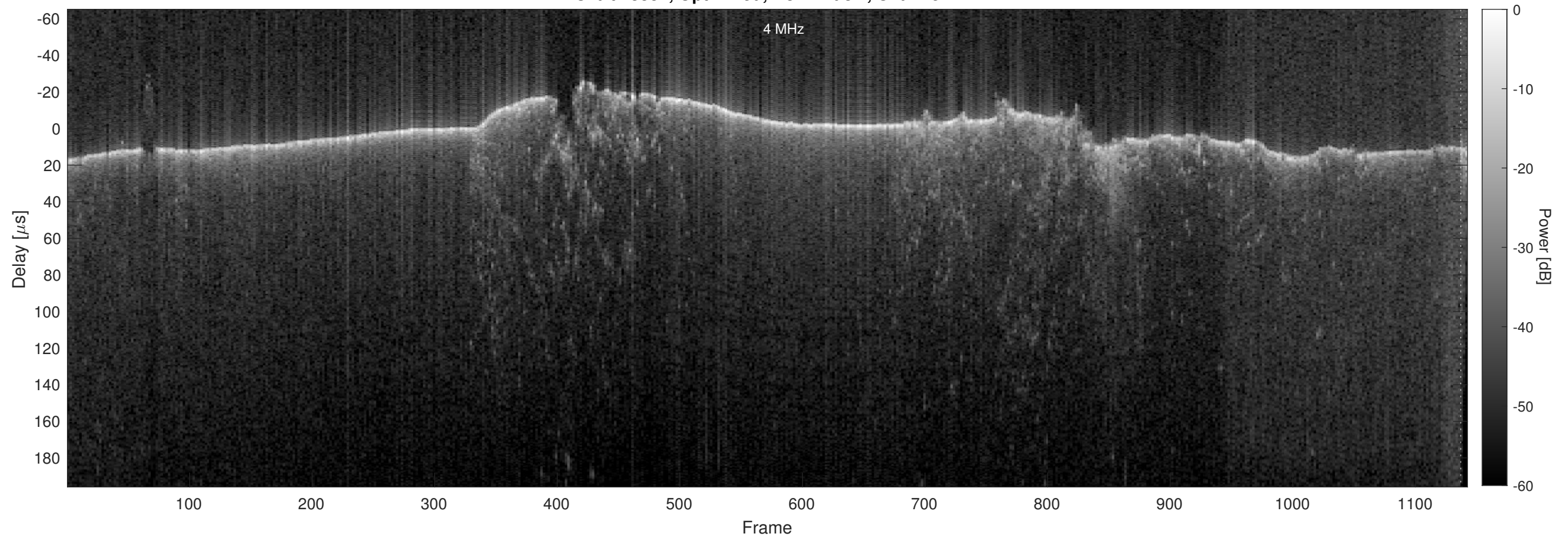
Orbit 13331, Optimized, No Window, Channel 2
