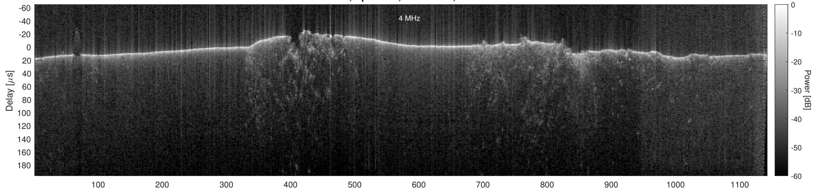
Orbit 13331, Optimized, No Window, Channel 2
