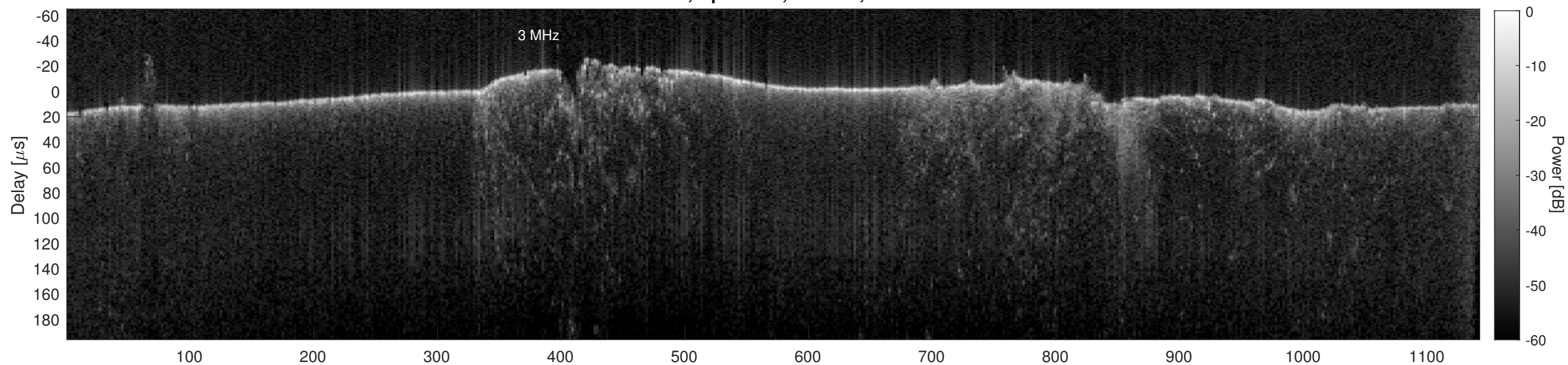
Orbit 13331, Cluttergram
