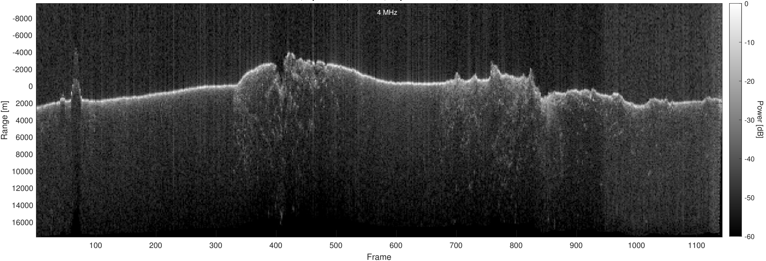
Orbit 13331, Optimized, Window, Depth-Corrected, Channel 2
