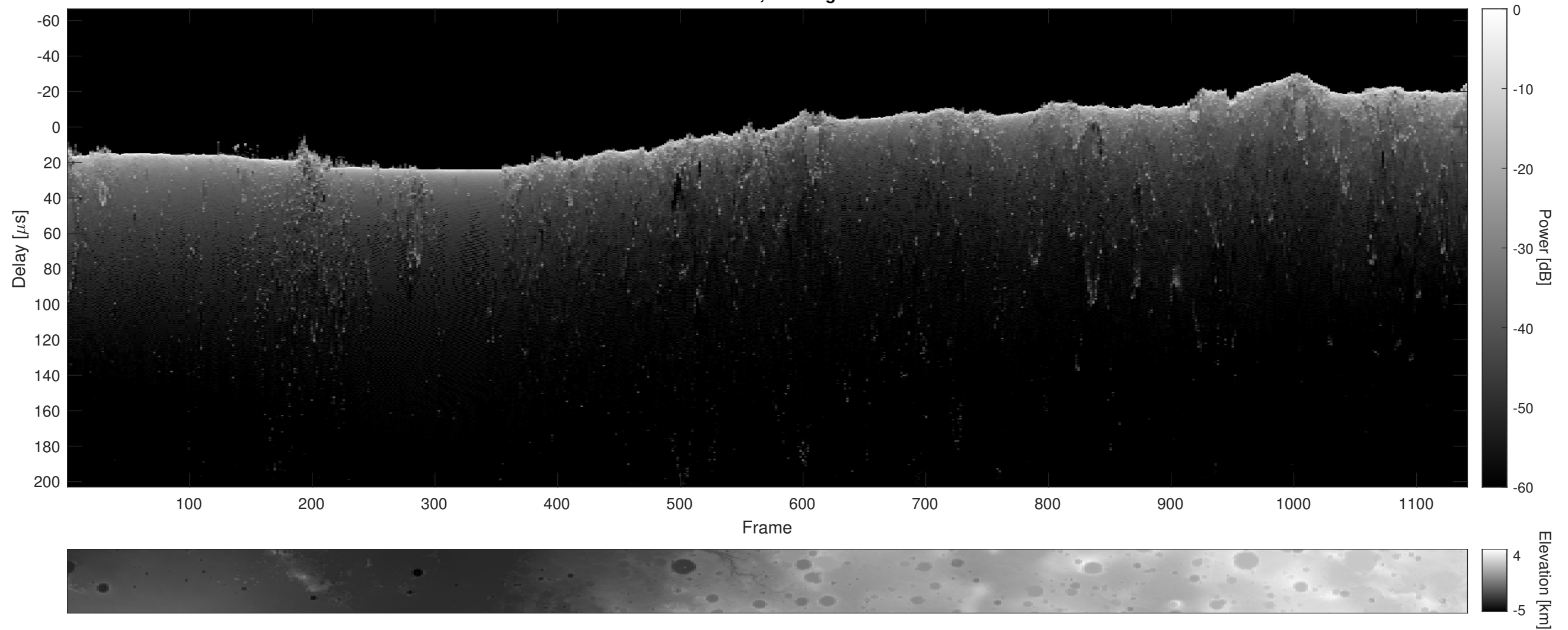
Orbit 13332, Cluttergram
