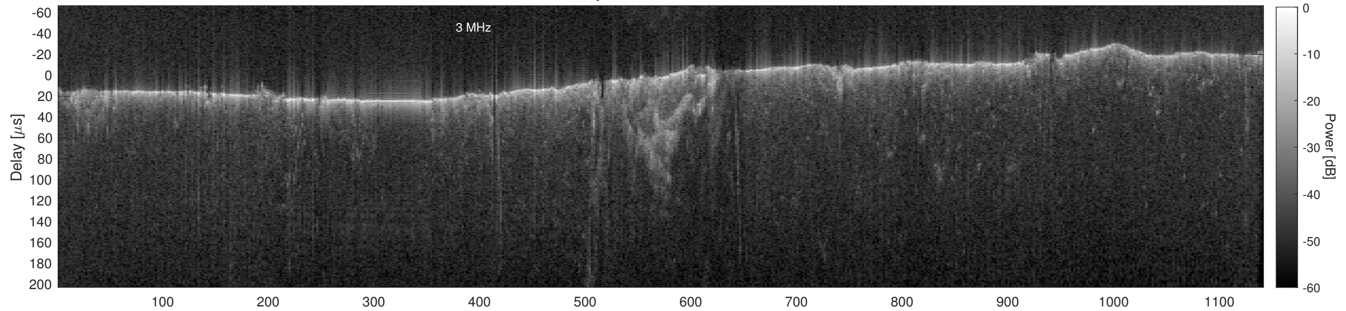
Orbit 13332, Cluttergram
