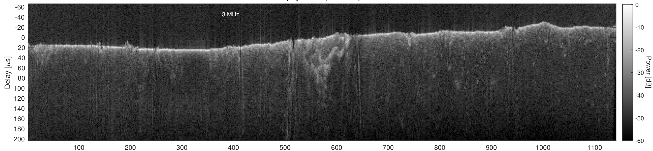
Orbit 13332, Cluttergram
