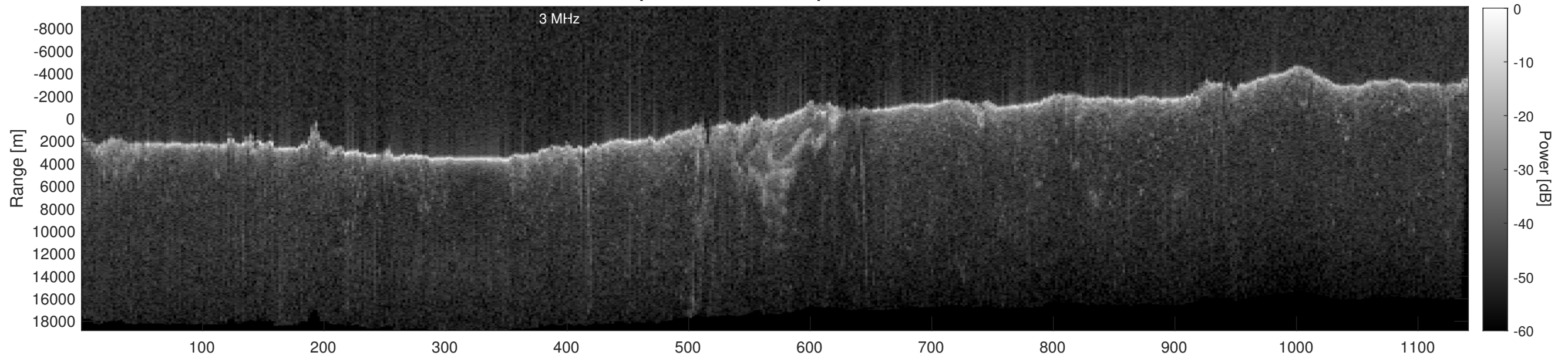
Orbit 13332, Depth-Corrected Cluttergram
