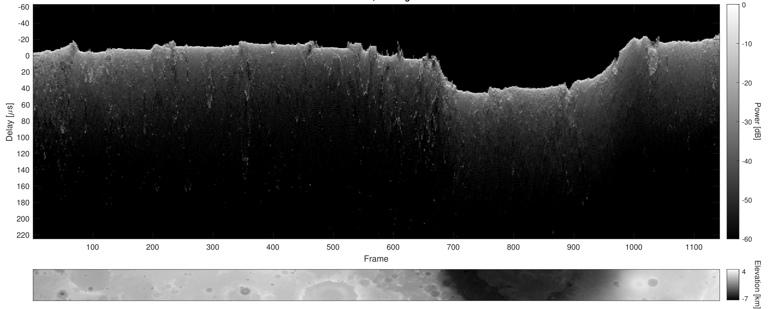
Orbit 13333, Cluttergram
