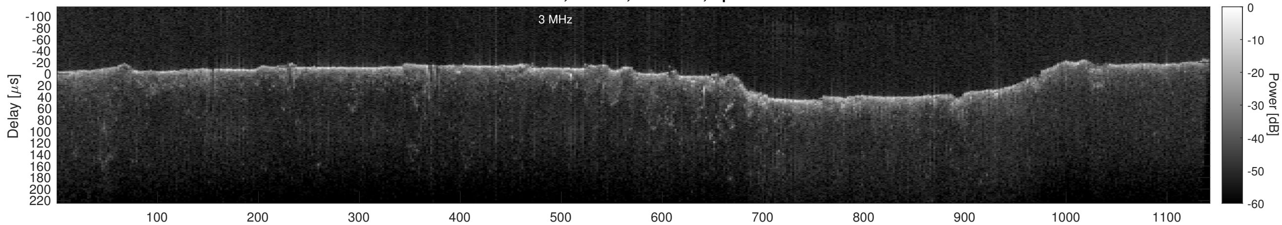
Orbit 13333, Cluttergram
