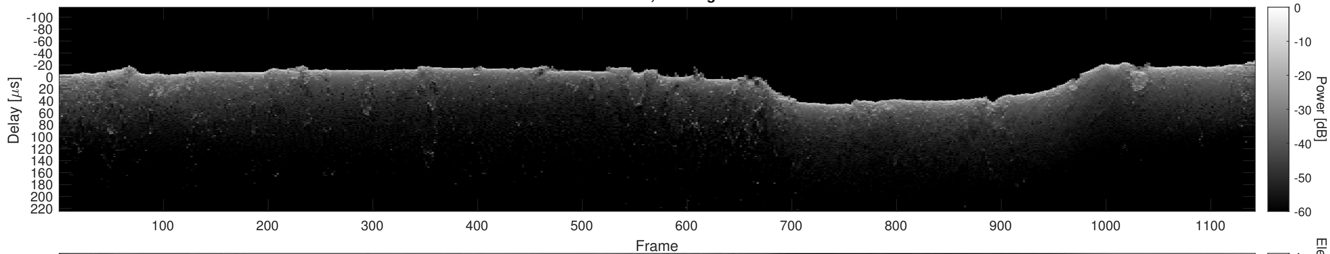
Orbit 13333, Cluttergram
