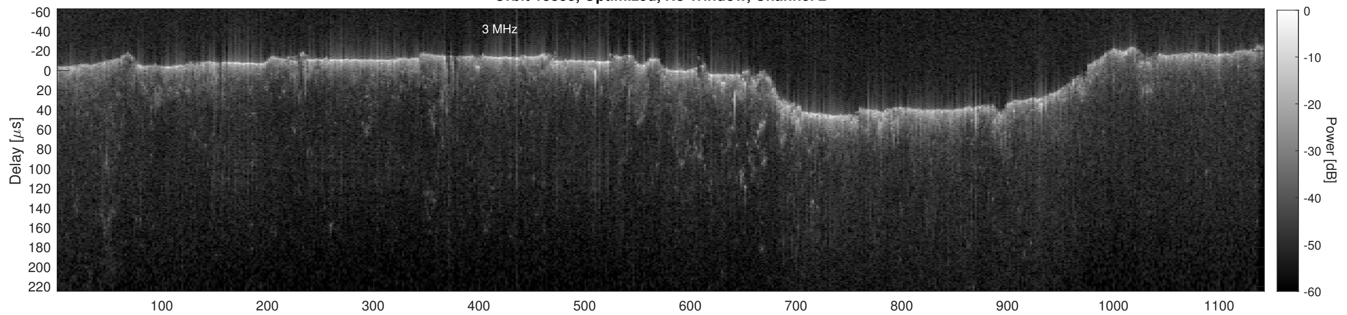
Orbit 13333, Cluttergram
