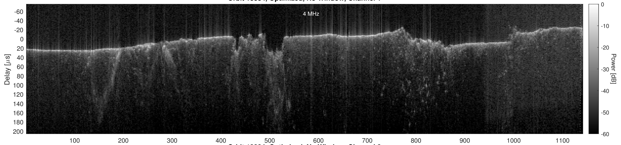
Orbit 13334, Optimized, No Window, Channel 2
