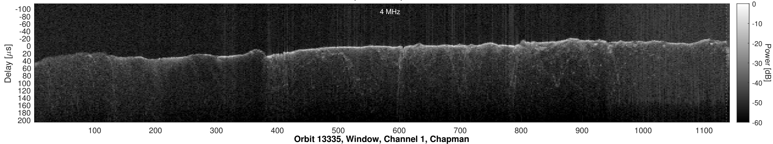
Orbit 13335, Channel 1, Uncorrected
