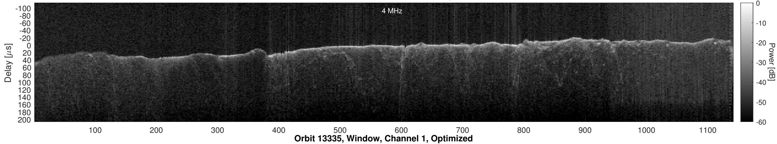
Orbit 13335, Window, Channel 1, Chapman
