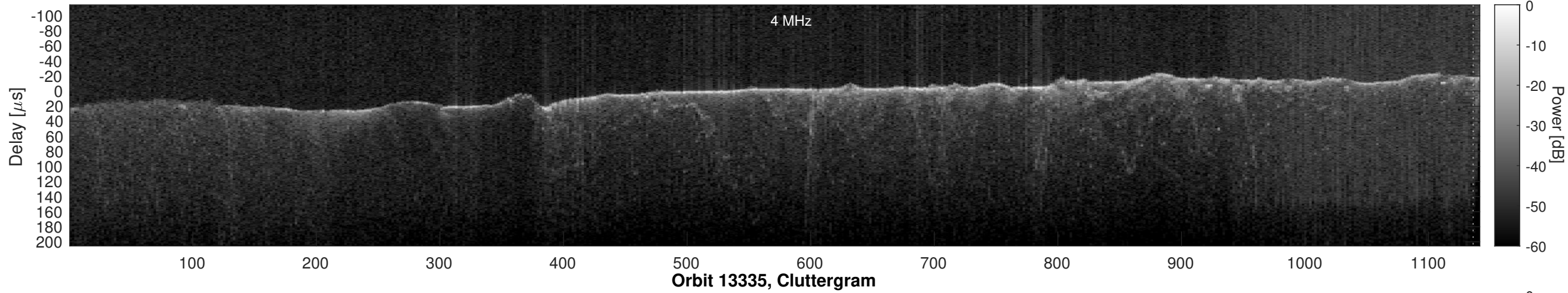
Orbit 13335, Window, Channel 1, Optimized
