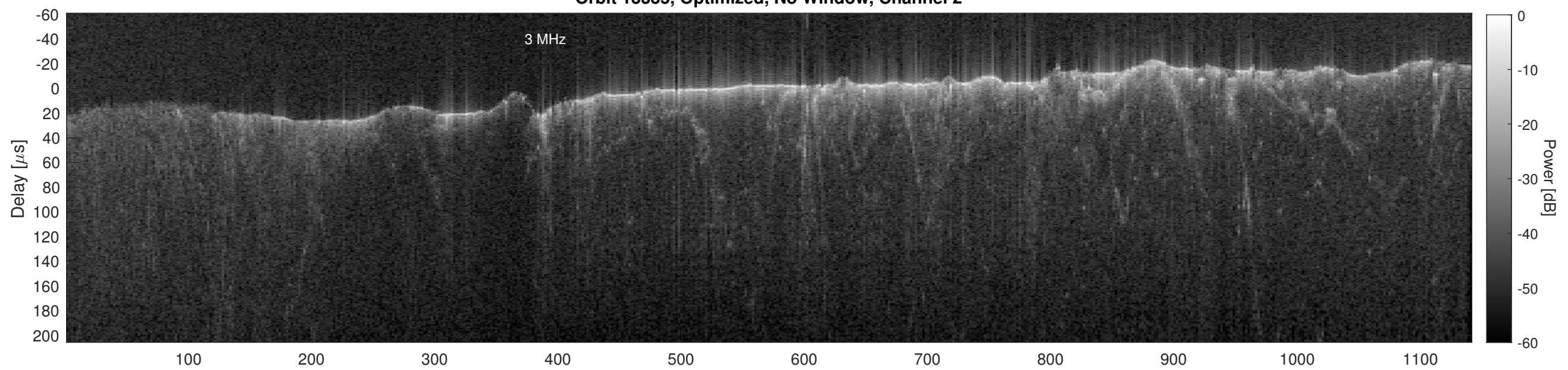
Orbit 13335, Cluttergram
