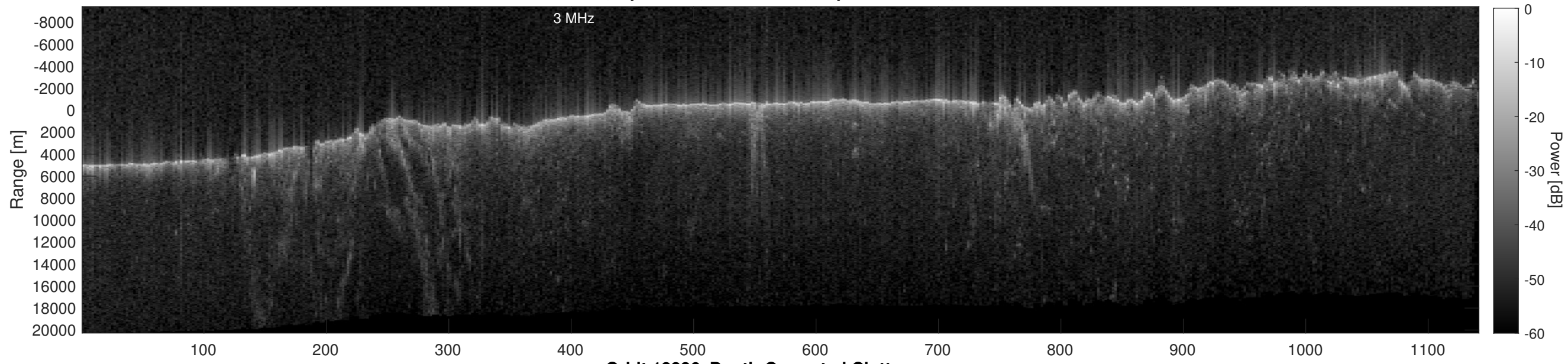
Orbit 13336, Depth-Corrected Cluttergram
