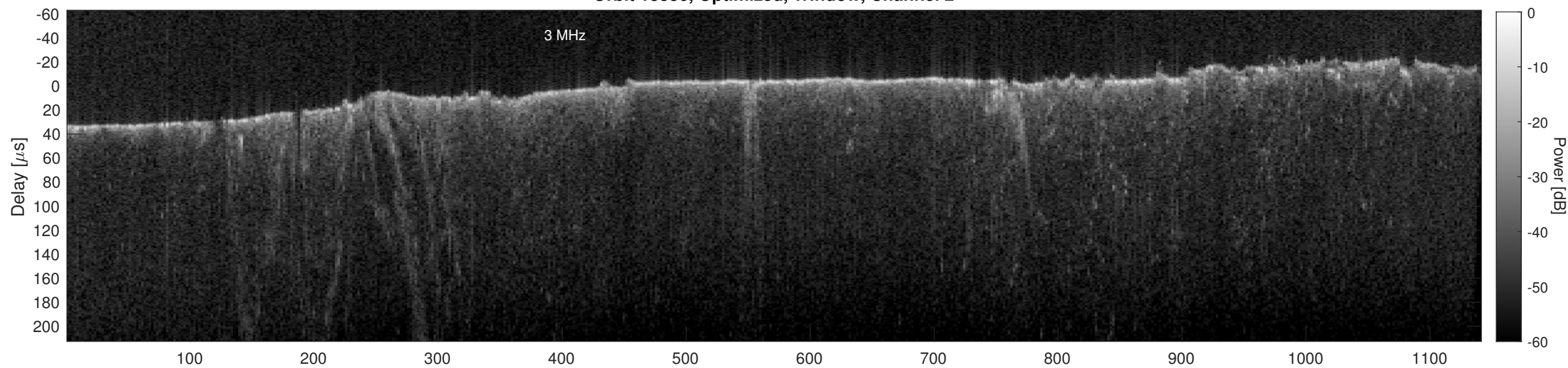
Orbit 13336, Cluttergram
