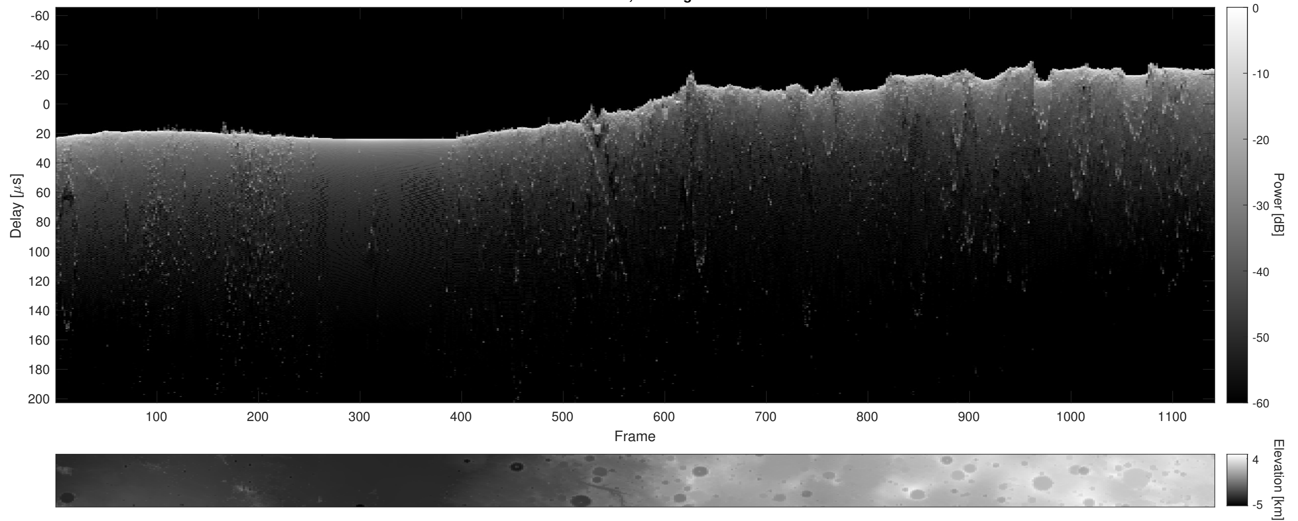
Orbit 13339, Cluttergram
