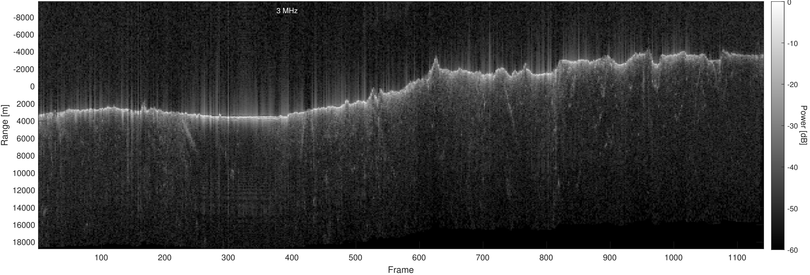
Orbit 13339, Optimized, No Window, Depth-Corrected, Channel 2
