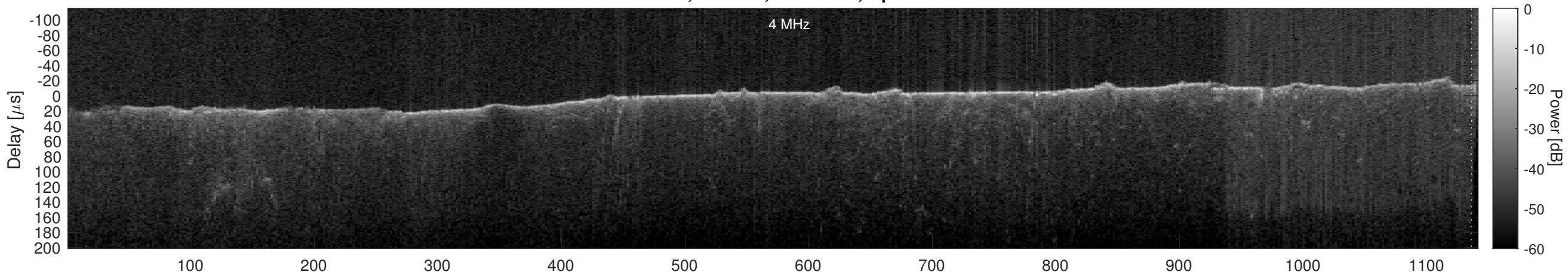
Orbit 13342, Cluttergram
