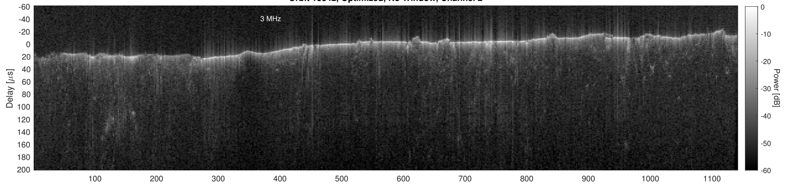
Orbit 13342, Cluttergram
