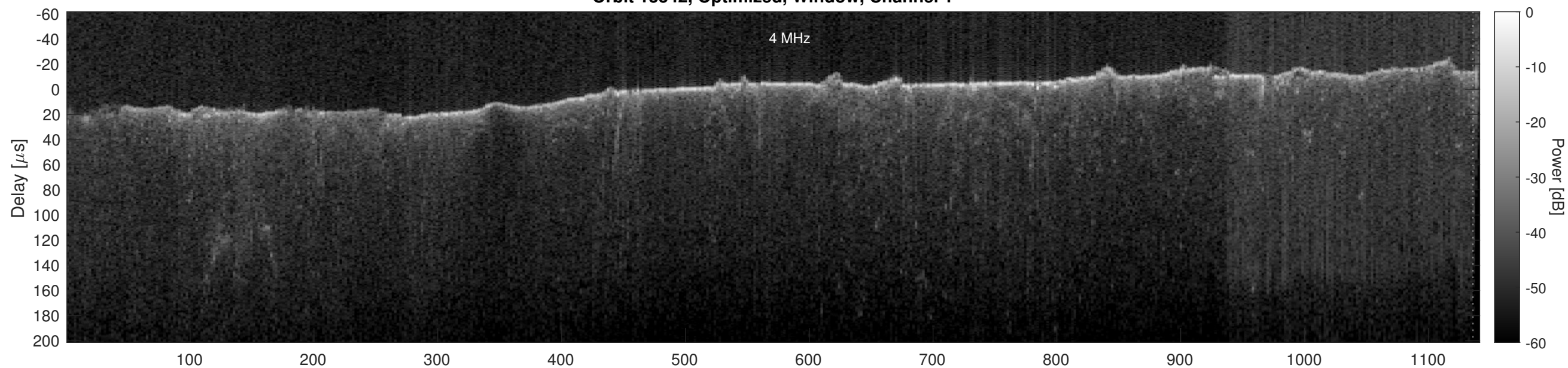
Orbit 13342, Optimized, Window, Channel 2
