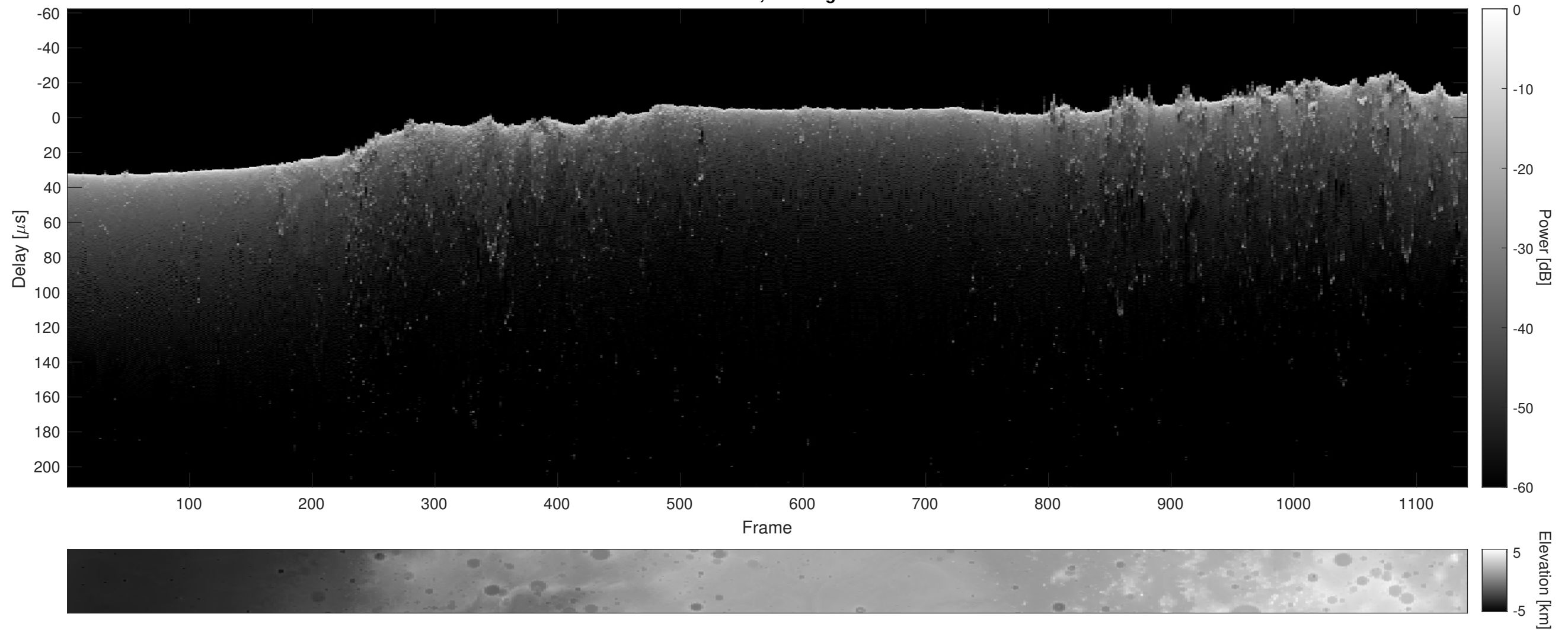
Orbit 13343, Cluttergram
