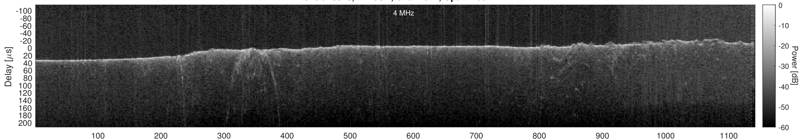
Orbit 13343, Cluttergram
