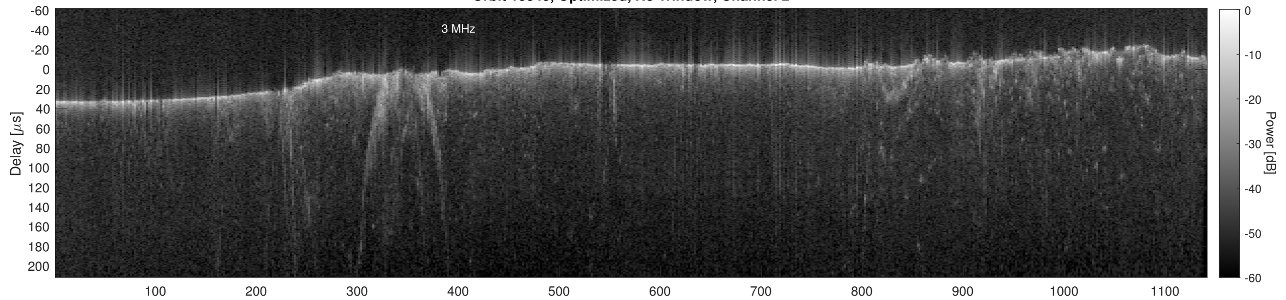
Orbit 13343, Cluttergram
