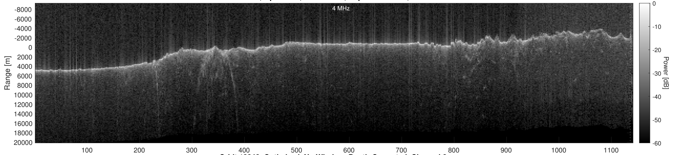
Orbit 13343, Optimized, No Window, Depth-Corrected, Channel 2
