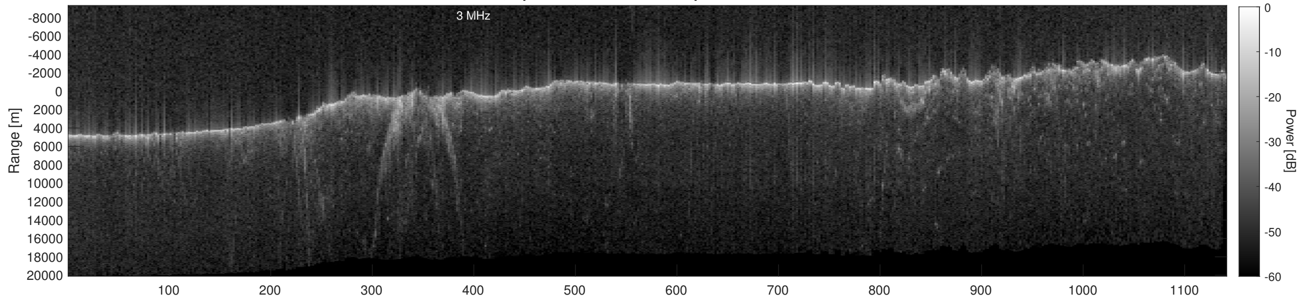
Orbit 13343, Depth-Corrected Cluttergram
