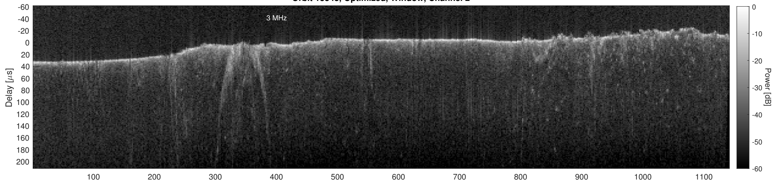
Orbit 13343, Cluttergram
