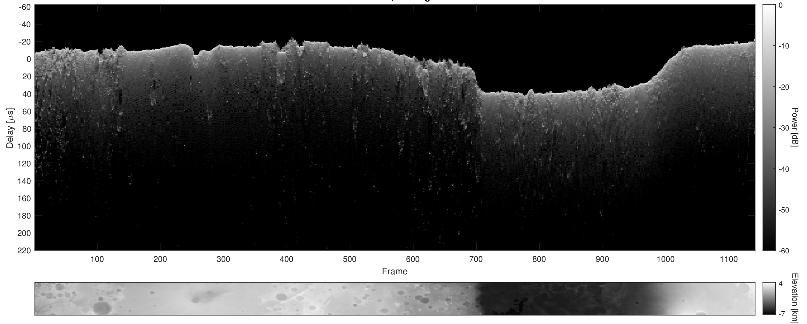
Orbit 13347, Cluttergram
