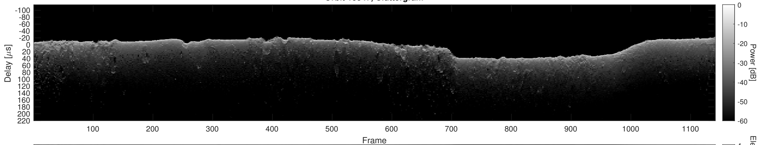
Orbit 13347, Cluttergram
