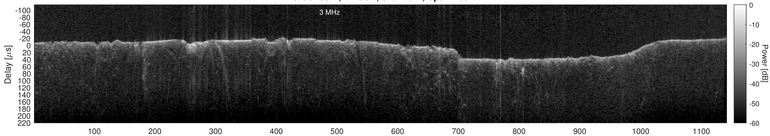
Orbit 13347, Cluttergram
