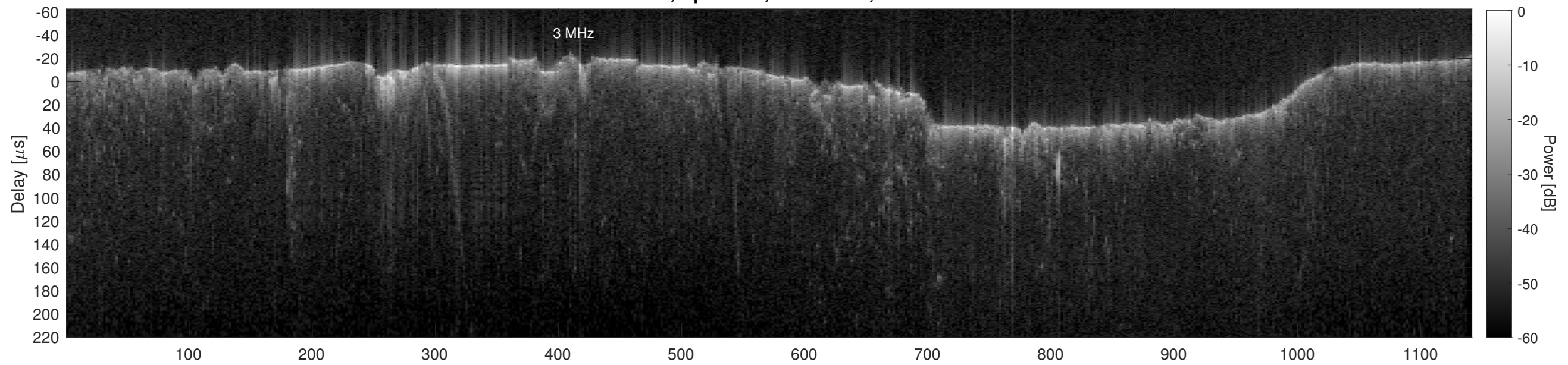
Orbit 13347, Cluttergram
