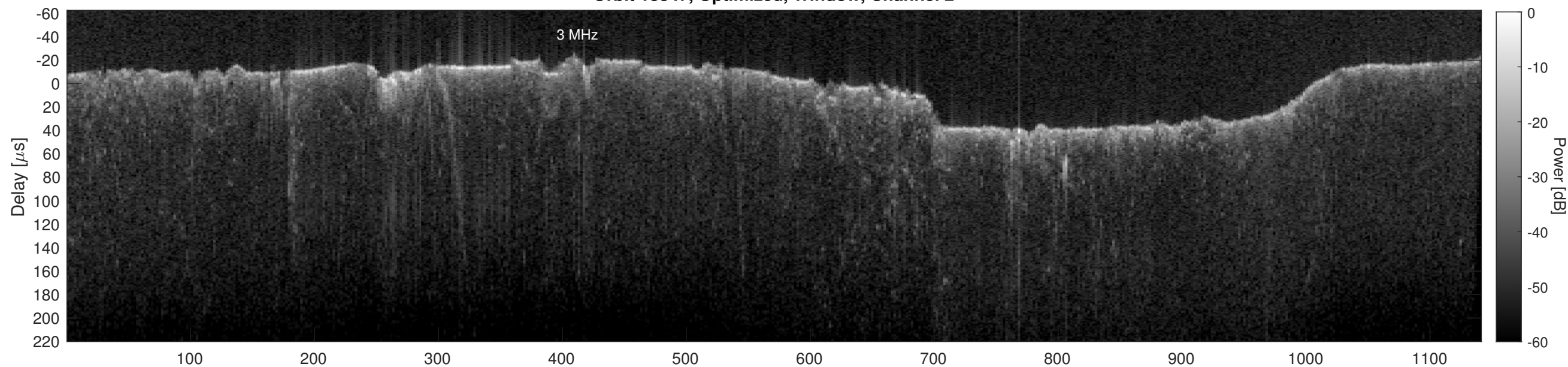
Orbit 13347, Cluttergram
