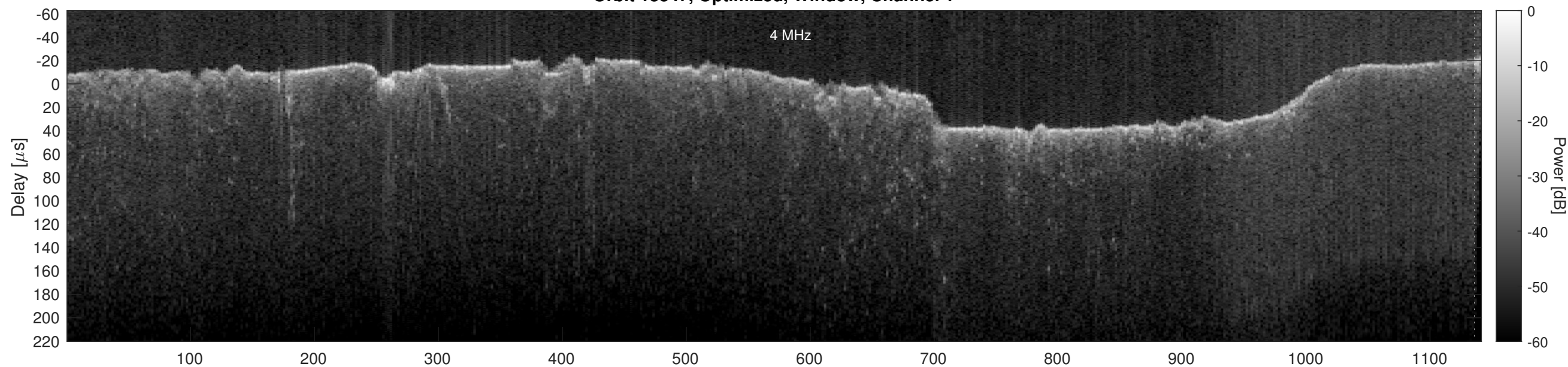
Orbit 13347, Optimized, Window, Channel 2
