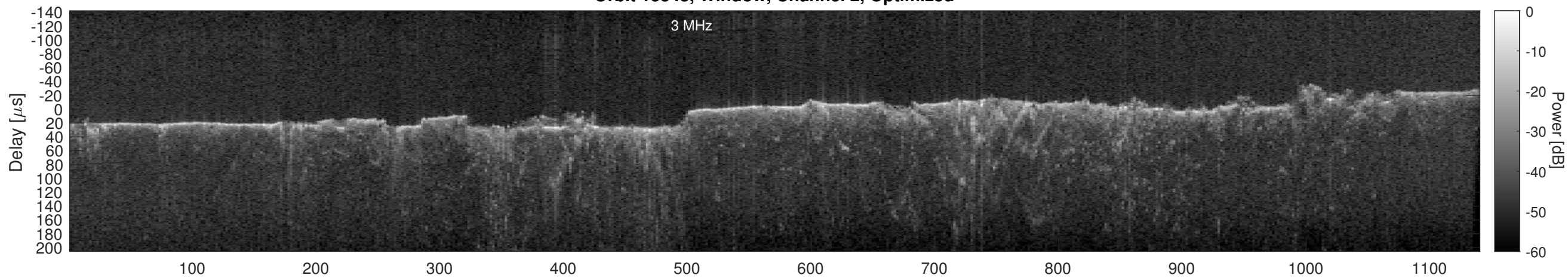
Orbit 13348, Cluttergram
