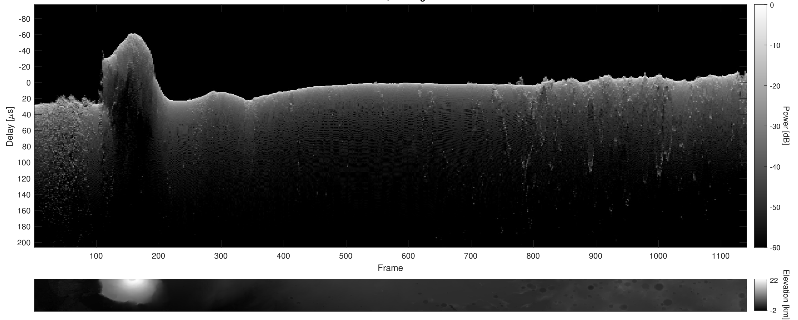
Orbit 13349, Cluttergram
