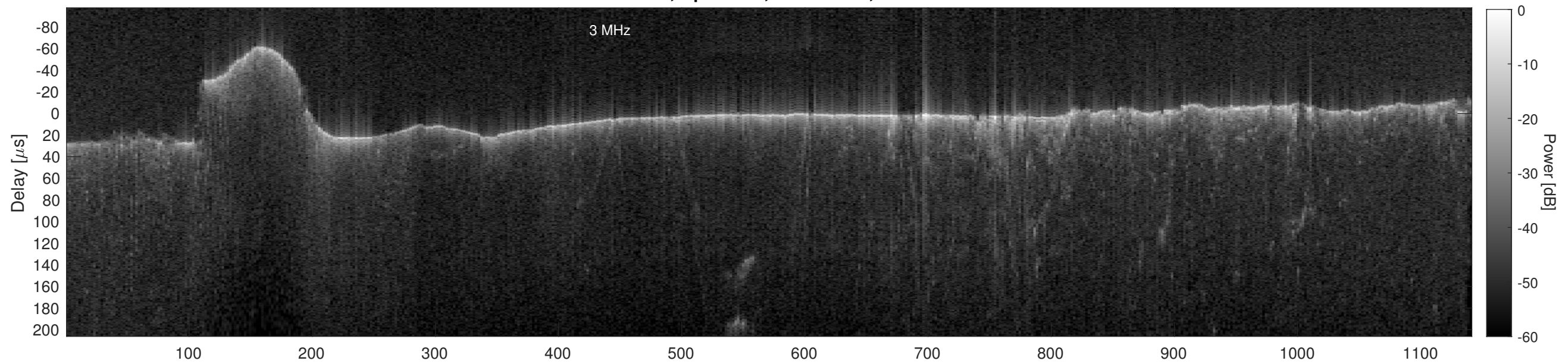
Orbit 13349, Cluttergram
