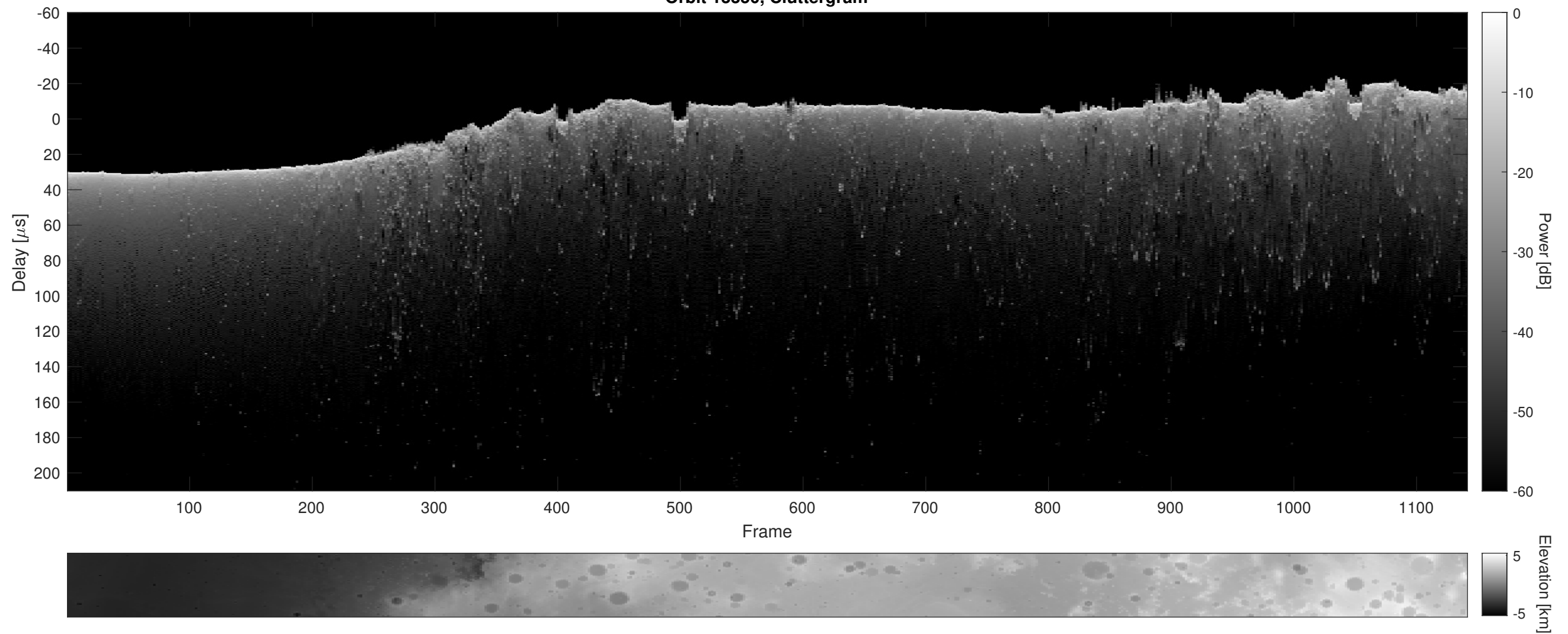
Orbit 13350, Cluttergram
