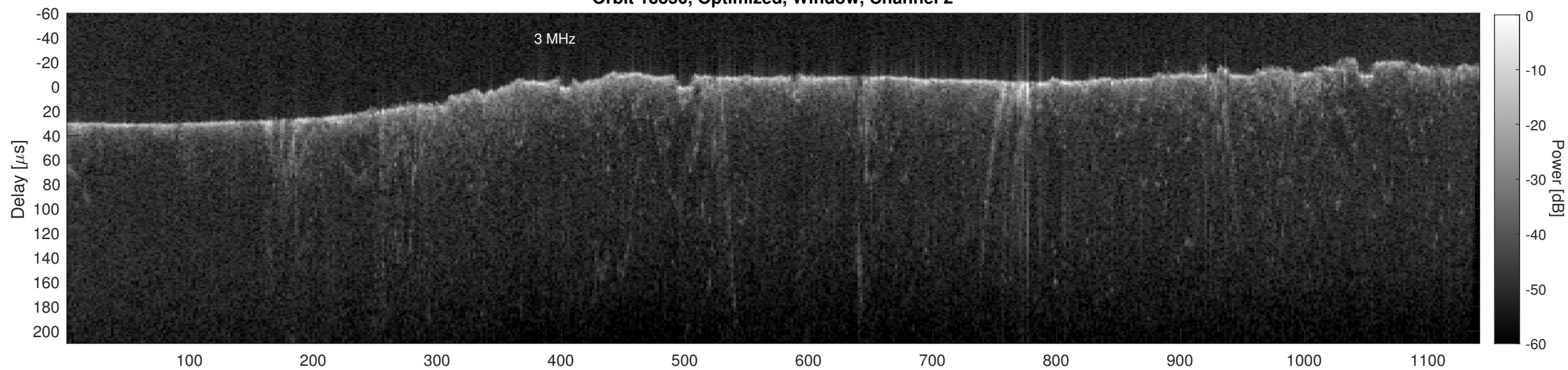
Orbit 13350, Cluttergram
