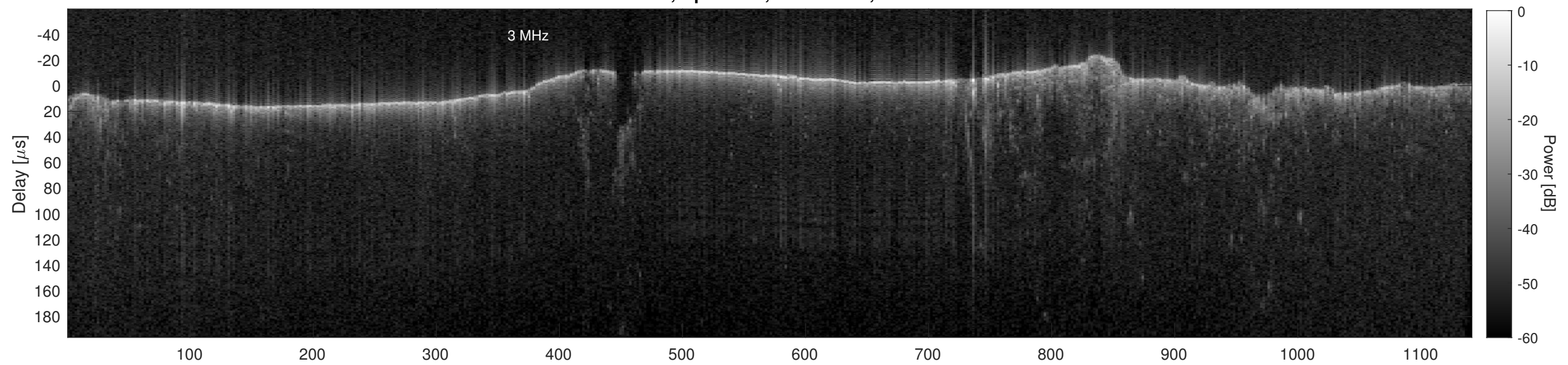
Orbit 13352, Cluttergram
