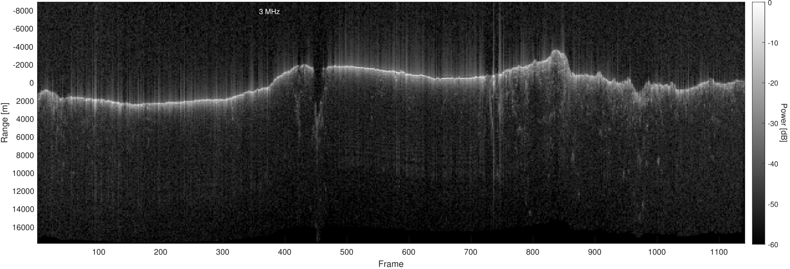
Orbit 13352, Optimized, No Window, Depth-Corrected, Channel 2
