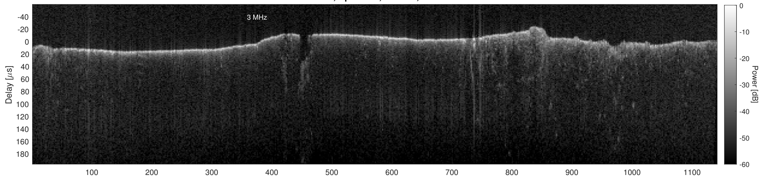
Orbit 13352, Cluttergram
