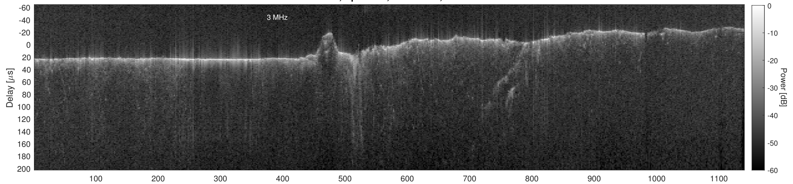
Orbit 13353, Cluttergram
