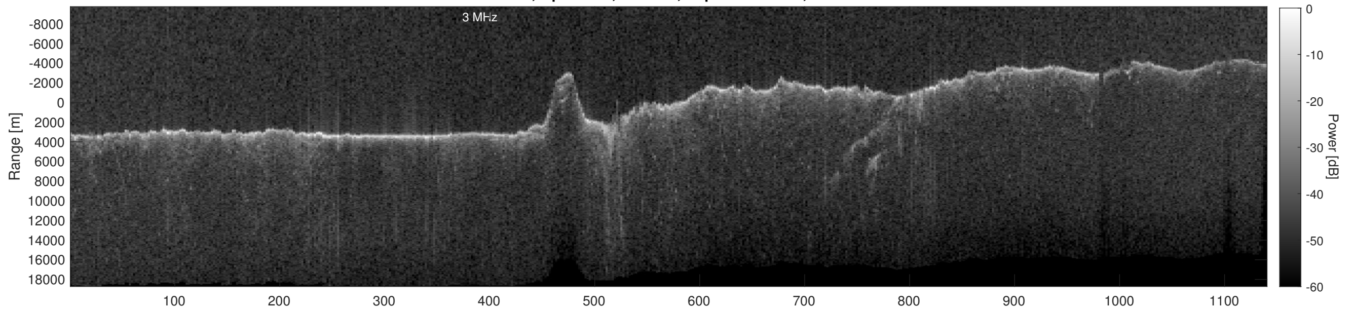
Orbit 13353, Depth-Corrected Cluttergram
