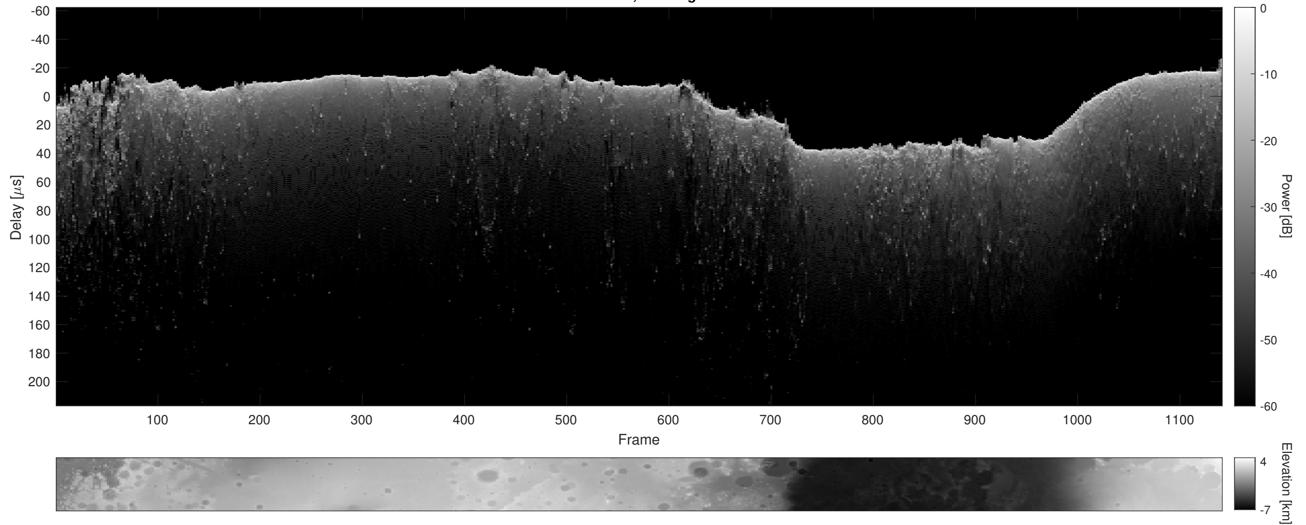
Orbit 13354, Cluttergram
